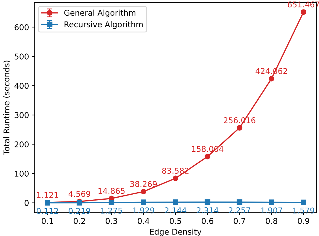
Total Runtime without Basis Tracking (200 realizations per density)
